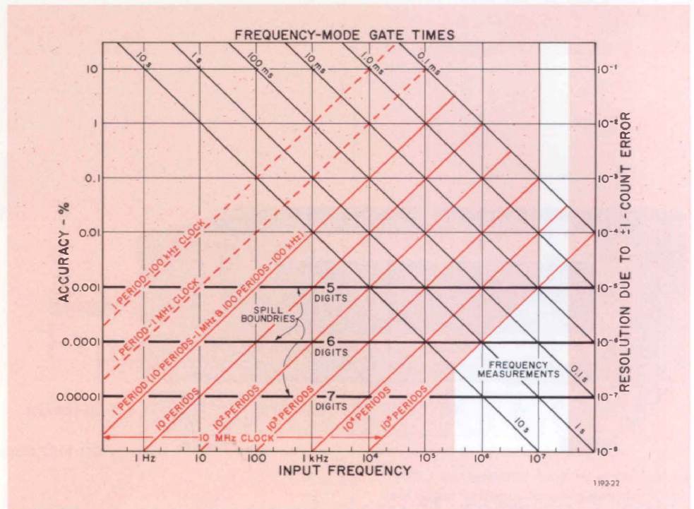
Figure 1. A summary of the GR 1192 resolution and display characteristics in its PERIOD and FREQUENCY modes. Within the white area resolution is highest in the FREQUENCY mode. The 1-ms GATE TIME prevents spill-over at the highest counting frequency; for period measurements, the 100-kHz counter clock permits up to 1-s periods to be measured without spill-over in the 5-digit counter, while the 10^5 -PERIODS control permits parts-per-million resolution at an input frequency of 1 MHz.
