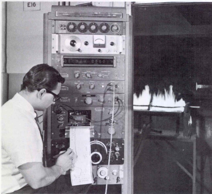
Figure 3. Test assembly for fire-resistant cables.
