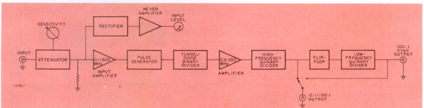
Figure 1. Block diagram of the GR 1157-B.
