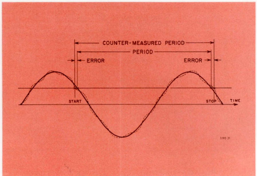
Figure 4. Effect of internal counter noise upon trigger point.
