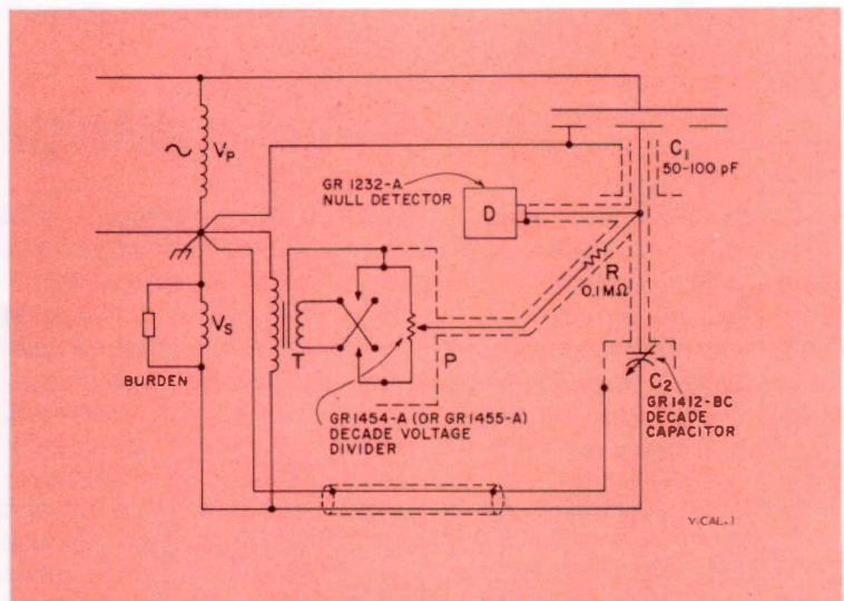
Figure 1. Schematic diagram of high-voltage transformer calibration circuit.
